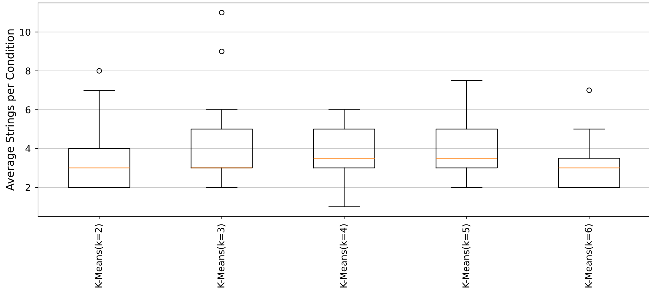
YARA Rules Average Strings per Condition Distribution (Cluster29_Size6 dataset)
